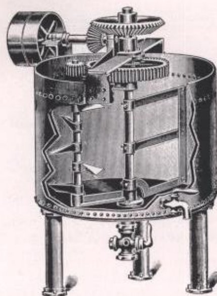
JACKETED STEAM MIXER.
