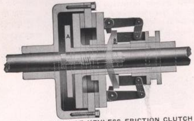
SECTIONAL VIEW OF KEYLESS FRICTION CLUTCH A.—Taper Sleeve. B.—Equalizing Adjusting Yoke. Dimensions of Standard Clutches.
