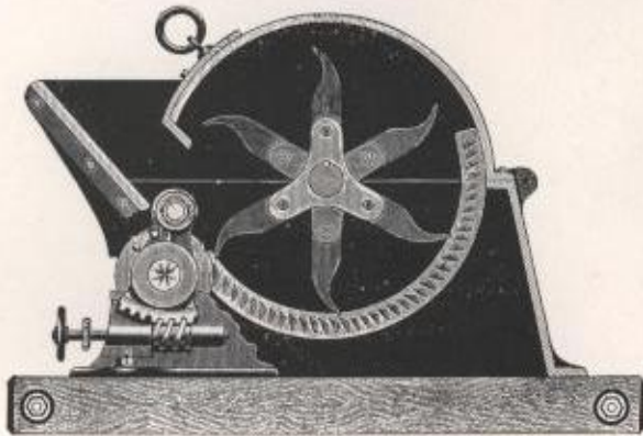
SECTIONAL VIEW.
