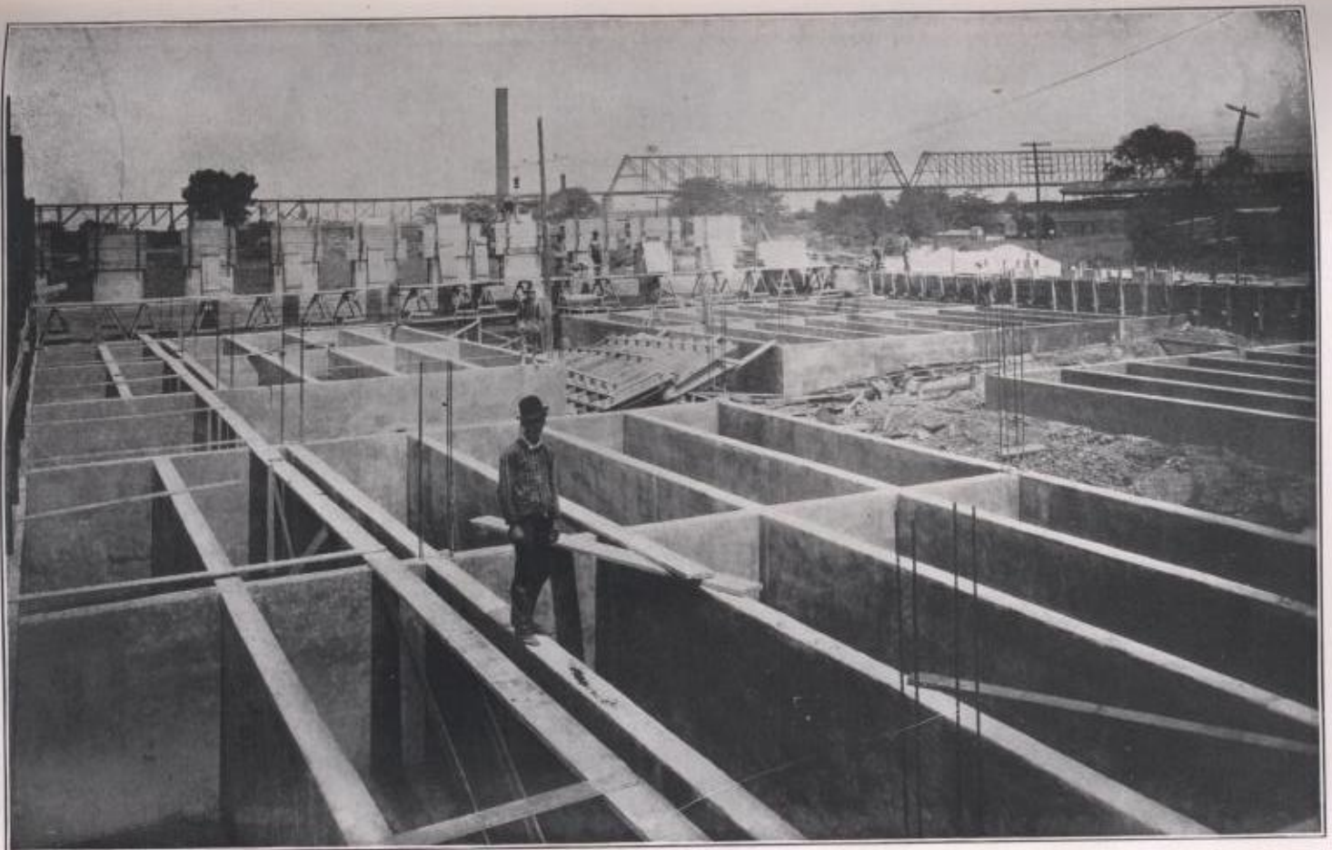
CONCRETE VATS. Showing the Construction of Vats before Building was Erected.
